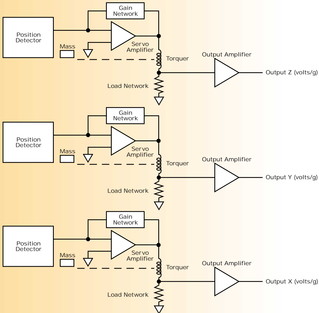
Block Diagram for the LCF Inclinometer
